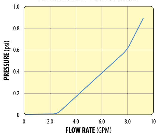
700 BARB Flow Rate vs. Pressure
