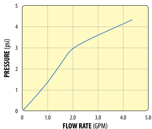
400 BARB Flow Rate vs. Pressure
