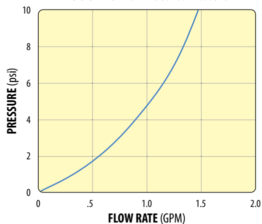
250 BARB Flow Rate vs. Pressure
